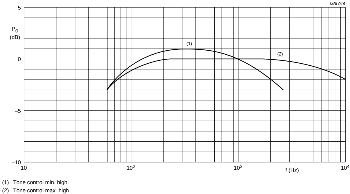
Fig.12 Frequency characteristics of the circuit of Fig. 10; P_O relative to 0 dB = 3 W; typical values.
