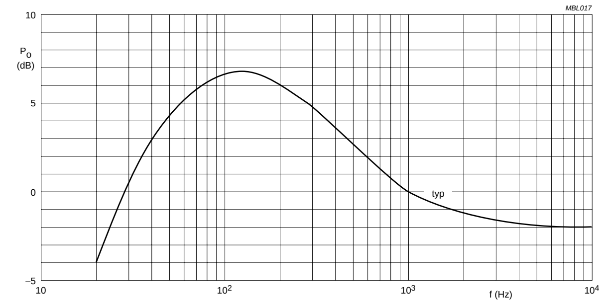
Fig.13 Frequency characteristic of the circuit of Fig. 10; volume control at the top; tone control max. high.
